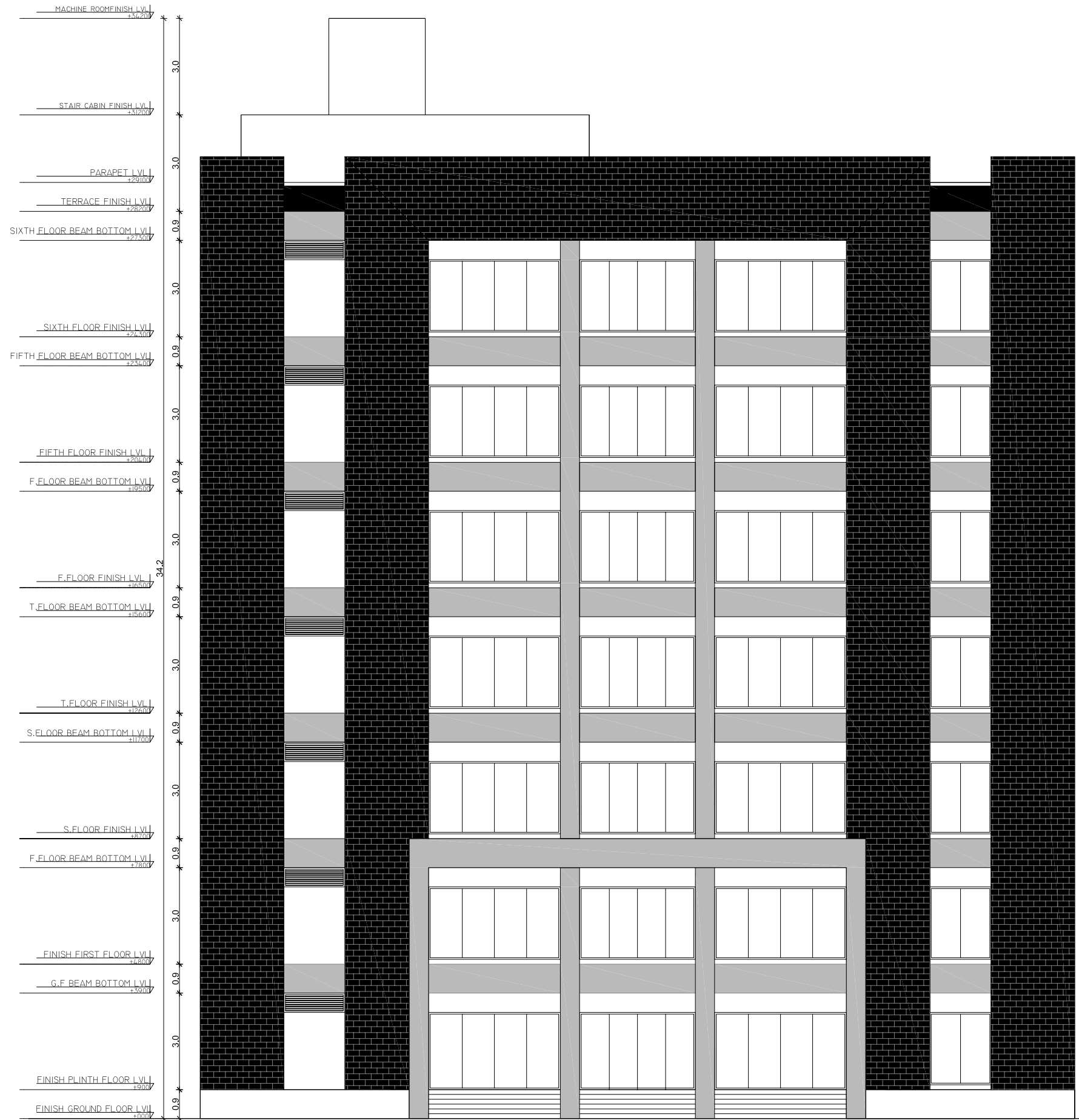
FRONT ELEVATION
